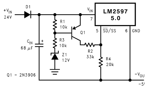
Figure 51. Undervoltage Lockout Without Hysteresis for an Inverting Regulator
