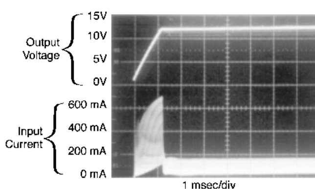
Figure 46. Output Voltage, Input Current, at Start-Up, WITHOUT Soft-start
