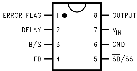
Figure 2. 8-Lead PDIP (P) Top View See Package Number P008E
