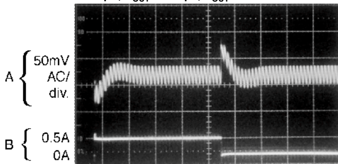
A: Output Voltage, 50 mV/div. (AC) B: 200 mA to 500 mA Load Pulse
