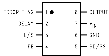
Figure 3. 8-Lead Surface Mount (D) Top View See Package Number D008A
