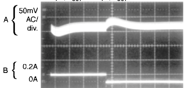
A: Output Voltage, 50 mV/div. (AC) B: 100 mA to 200 mA Load Pulse
